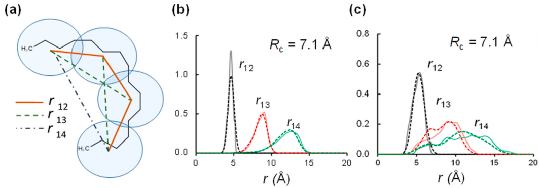
Fig. 6. (a) Nearest ( r_{12} ), second nearest ( r_{13} ) and third nearest r_{14} neighbor distances in a polymer chain. (b) Distributions of r_{12} , r_{13} and r_{14} for n-alkanes in atomistic MD (solid) simulations and DPD (dashed) simulations at the CG level corresponding to R_C = 0.71 \text{ nm} . (c) Distributions of the same for PEO. (Adapted with permission from Lee et al. ref. [42], Copyright 2016, American Chemical Society.). (For interpretation of the references to color in this figure legend, the reader is referred to the web version of this article.)
